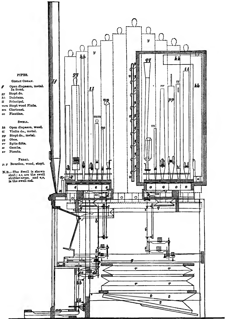
General Section of an Organ with two Manuals, Great and Swell, and Pedals.
